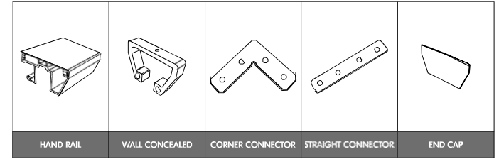
HR-13 (71x35mm LED)
